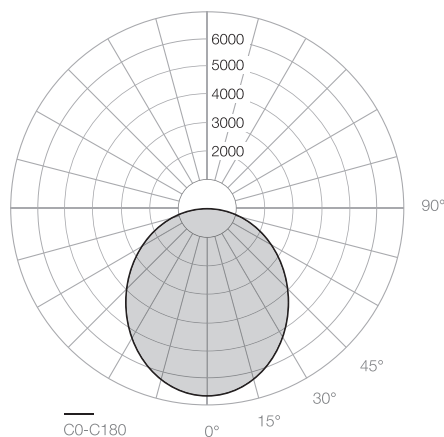
LIGHT DISTRIBUTION FOR 3000K
