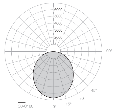
LIGHT DISTRIBUTION FOR 3000K
