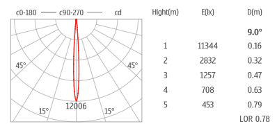
LIGHT DISTRIBUTION FOR 3000K
