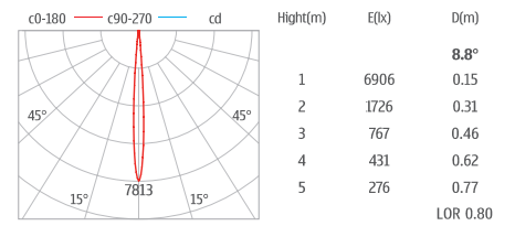
LIGHT DISTRIBUTION FOR 3000K
