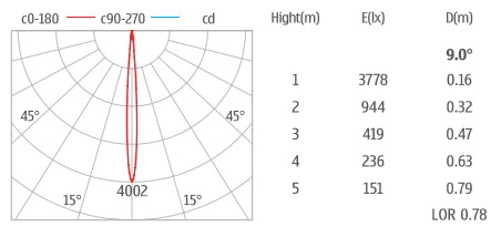
LIGHT DISTRIBUTION FOR 3000K
